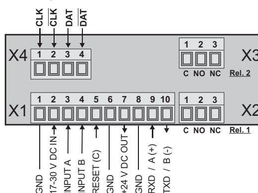
Display with 2 relay outputs, RS 232/485 (0.570.010.305)
