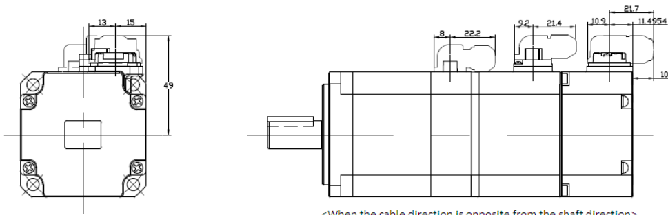
<When the cable direction is opposite from the shaft direction>
