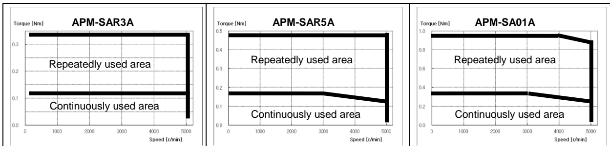
◆ Rotation Speed - Torque Characteristics ◆
