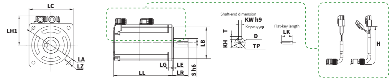
Connector-type
