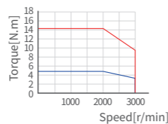
X2MM100A▲
