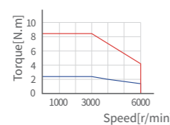
X6MH075A ▲
