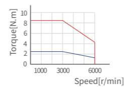
X6MH075H ▲
