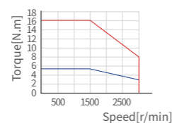
X6MG085S ▲
