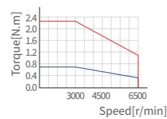
X6MH020H ▲
