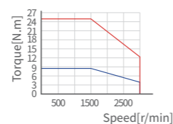
X6MG130S ▲
