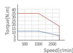
X6MG180S ▲
