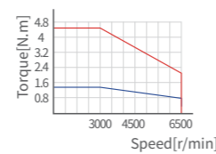
X6MH040H ▲
