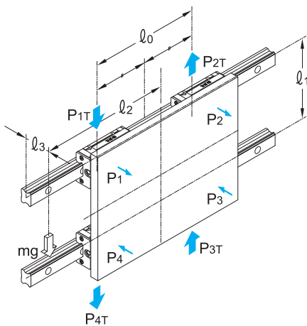
Condition 4 Vertical axis with wall mounted
