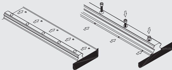
④ Final tightening of mounting bolts
